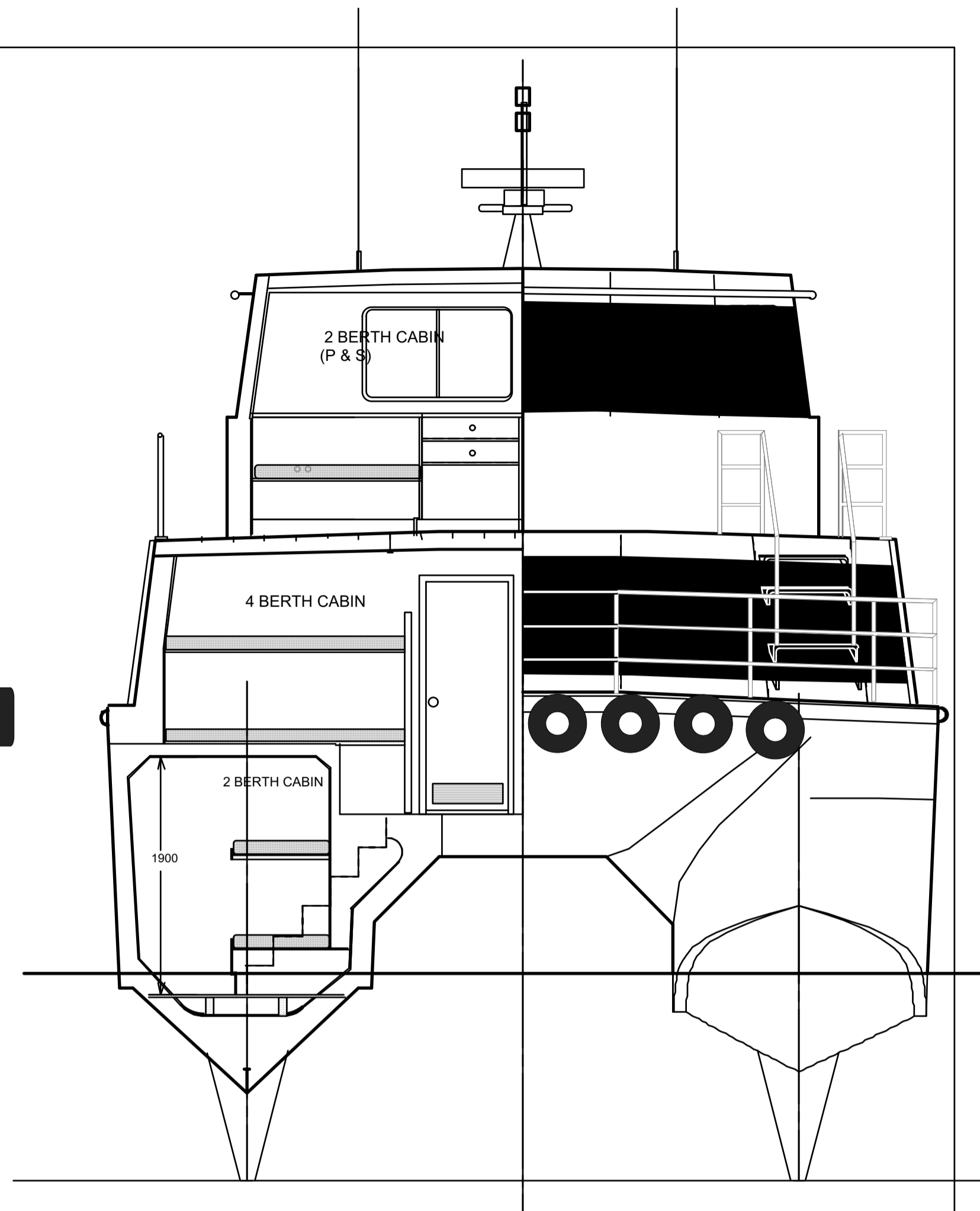
INTERNAL SECTION
