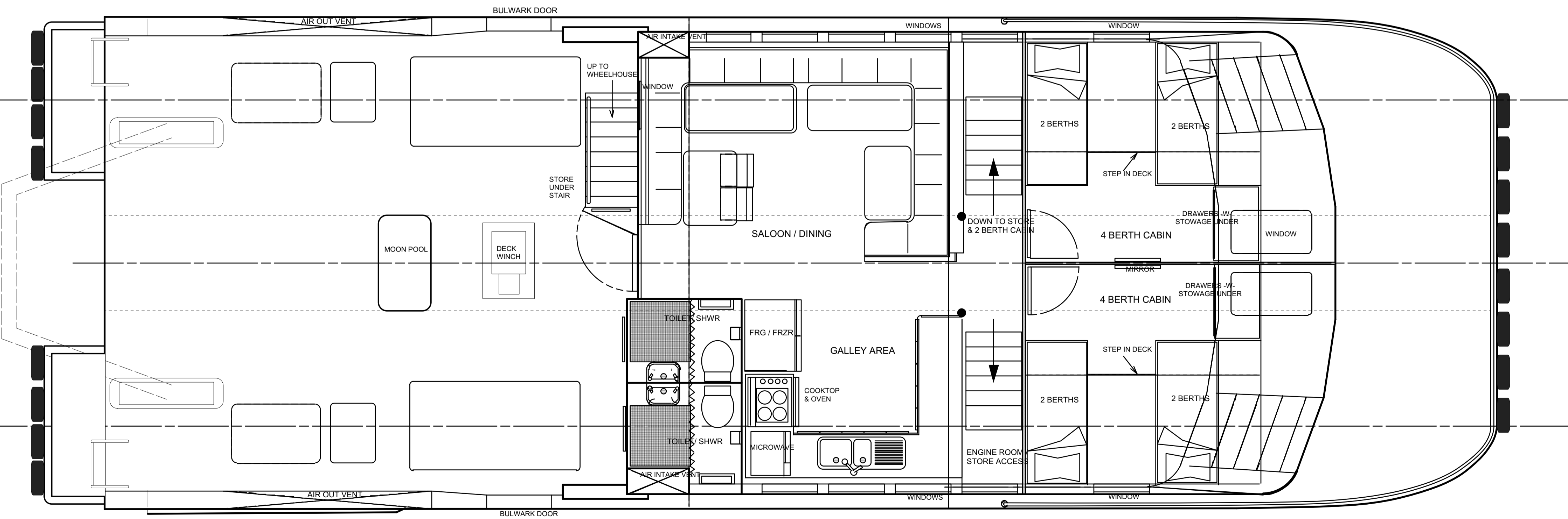
MAIN DECK PLAN
