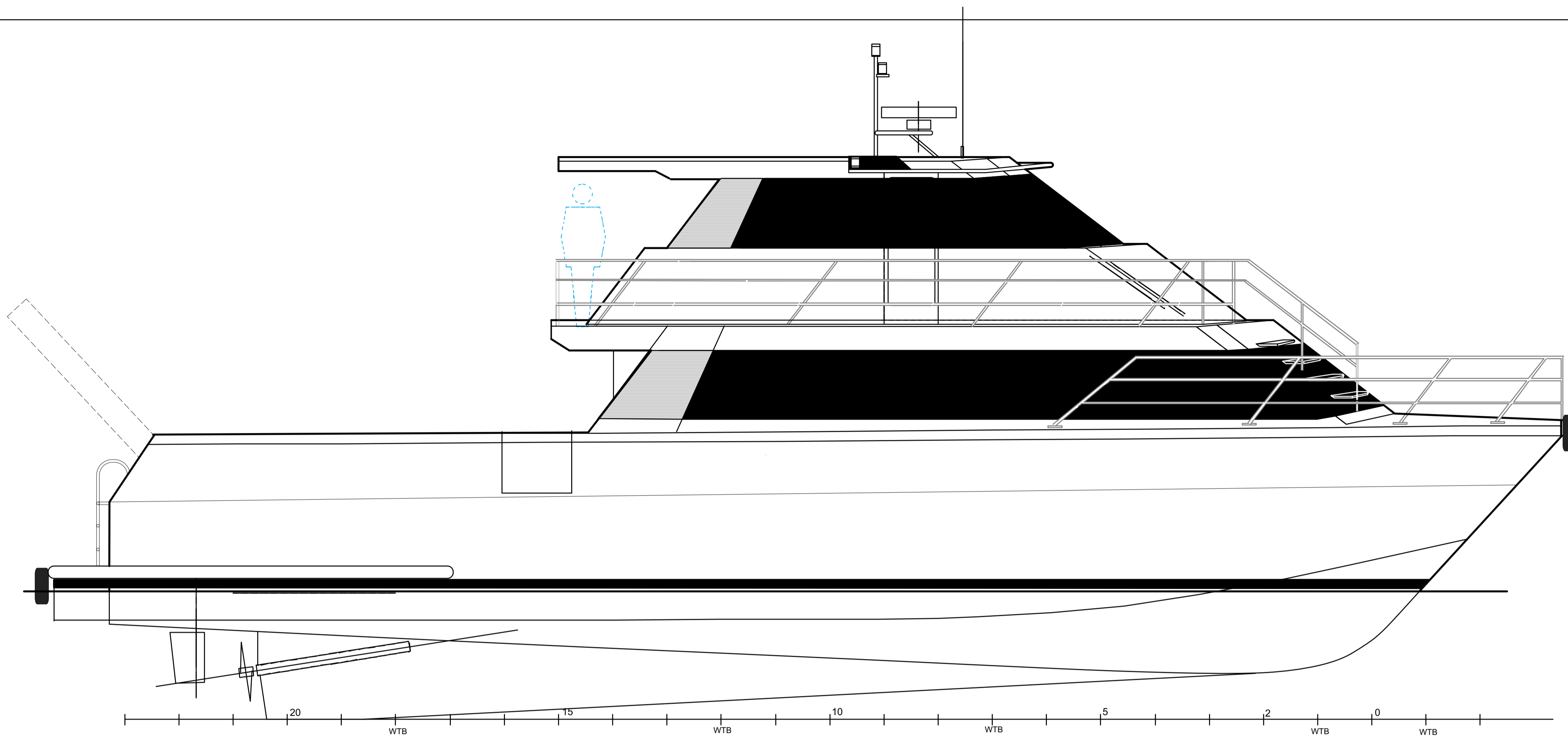
OUTBOARD PROFILE
